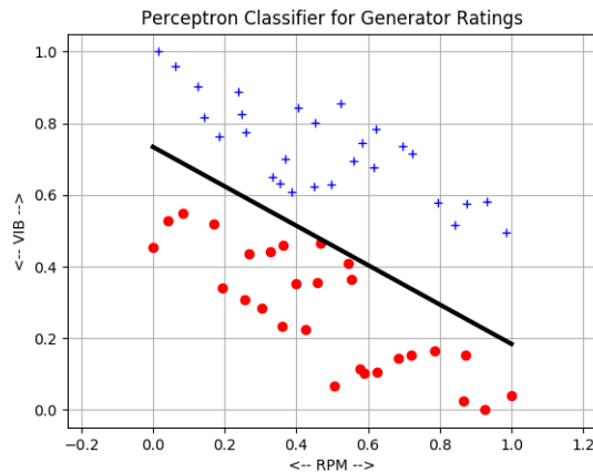
The dividing line produced by the perceptron algorithm
